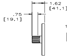
VIEW SHOWING OPTIONAL SPLINE SHAFT SAE INVOLUTE SPLINE 13 TEETH 16/32 PITCH .859 [21.82] MAJOR DIA. (INDUSTRIAL VERSION)
