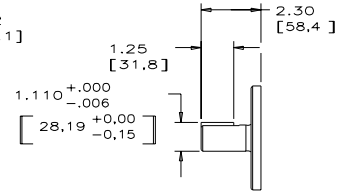
VIEW SHOWING OPTIONAL KEYED SHAFT ø1.000-.001 [25.40-.025] W/ .250 [6.35] SQ. KEY
