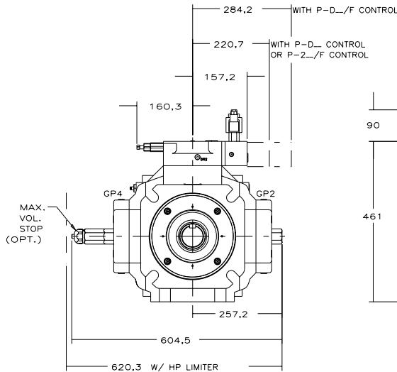
P-2_ CONTROL DUAL PRESSURE COMPENSATOR CONTROL
